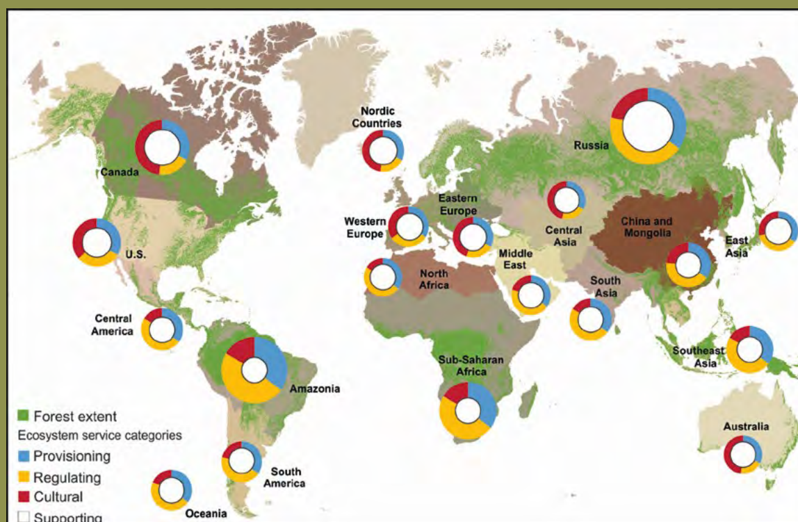
Figure 5.2. Map illustrating the portfolio and relative magnitude of ecosystem services provided by forests. The relative magnitude of ecosystem services for each region is illustrated by the relative size of the circles, whereas the relative size of each segment represents the value of each service
