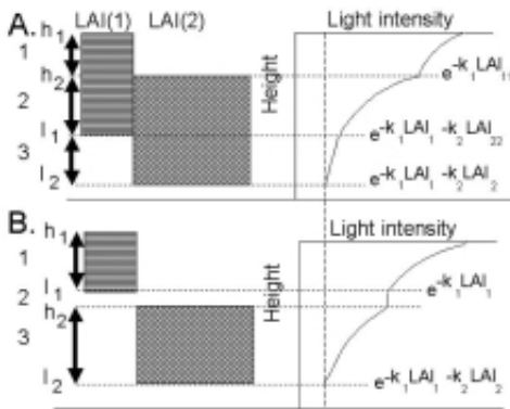
Figure 3.19. Light capture in a two-component leaf canopy, as used in WaNuLCAS 1.0; three zones can be distinguished: an upper zone with only one species, a middle one with both and a lower one with only one (usually not the same as in the upper zone); total light capture in the shared zone may be apportioned relative to the leaf area index of both species in that zone (compare Kropff and Van Laar, 1993)
