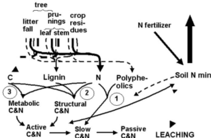
Figure 3.30. Major relationships in N immobilization and N mineralization from organic residues; the basic C and N pools are similar to the Century model, but plant polyphenolics are added as litter quality parameter
