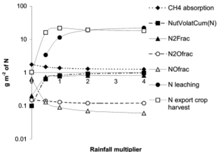
Figure 3.15. Effect of total rainfall, as simulated by using multiplier on daily rainfall amounts, on the gaseous N emissions from a soil (specified over \text{NO} and \text{N}_2\text{O} ), leaching and N export from the plot in crop harvests over a 5 year period
