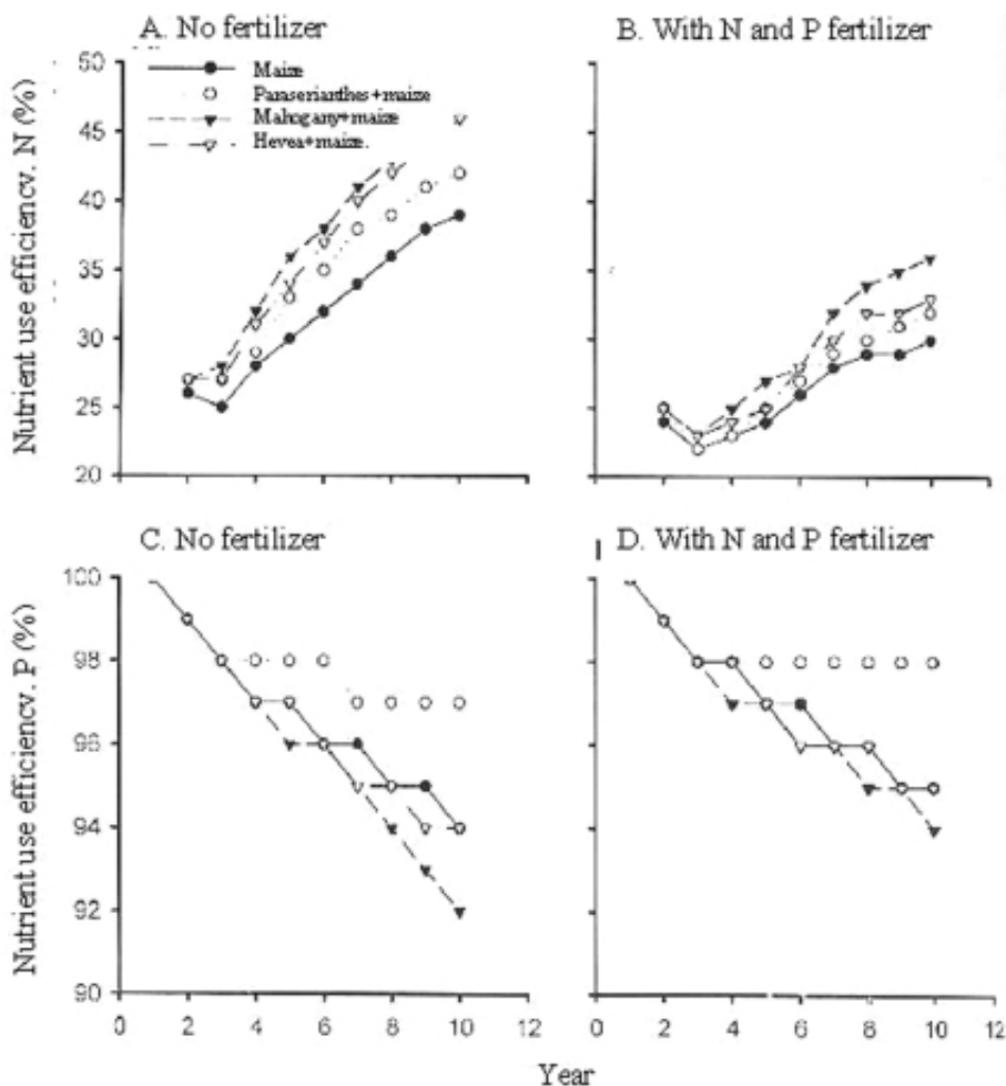
Figure 4.12 Nutrient (N and P) use efficiency in the different agroforestry systems: maize monoculture, paraserianthes + maize, mahogany + maize and hevea + maize. (A and C) no fertilizer and (B and D) with N and P fertilizer
