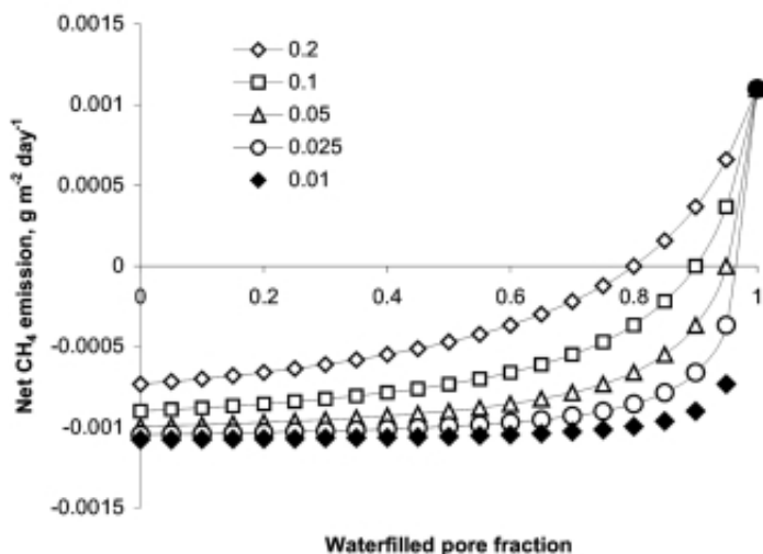
Figure 3.14. Methane flux (negative values indicate consumption, positive ones emission) as a function of the water-filled pore space, for a range of values of the \text{GHG\_CH}_4\text{\_Km} parameter (a dimension parameter relating to the difference in water-filled pore space (by decrease from fully saturated soil) that causes a 50% change in net emission, within the range defined by highest and lowest flux
