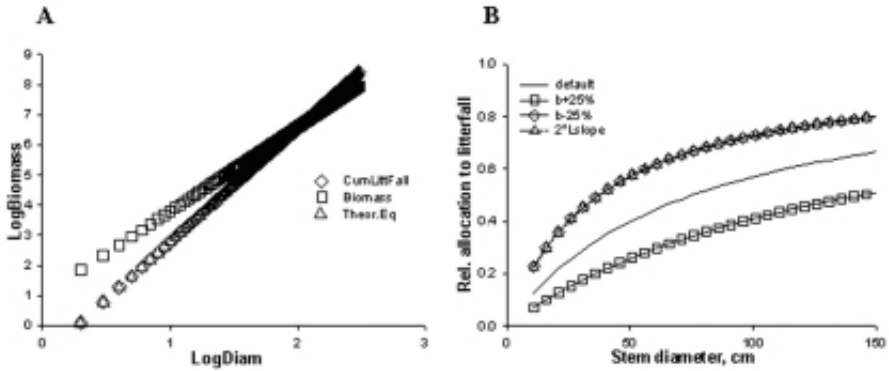
Figure 3.27. A. Comparison of biomass and cumulative litterfall as a function of stem diameter comparing a numerical integration with results of eq.[54]; B. Relative allocation of current biomass production to litterfall as a function of stem diameter for a default parameter set and in situations where the slope of the biomass allometric equation is increased or decreased by 25%
