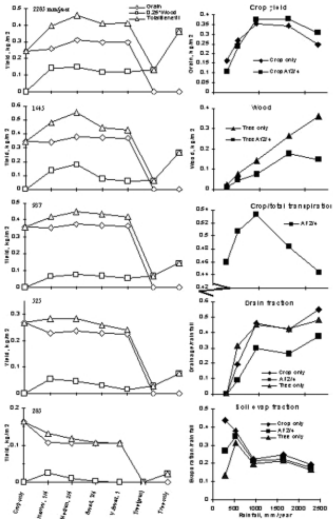
Figure 4.8 Calculations with the WaNuLCAS model of grain and wood production and water use for a range of annual rainfall conditions in an agroforestry system with isolated trees which are pruned when a crop is sown, resembling an early stage of a parkland system; production is accumulated over 2 years, involving 4 (at 2285 and 1645 mm/year) or 2 crops of 98 days duration, on a sandy soil with limited N mineralization from soil organic matter (for main parameter settings see text)
