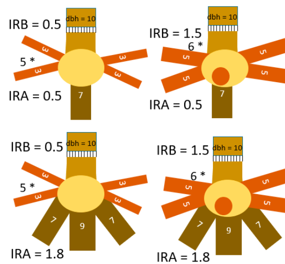
Figure 10. Examples of root-to-shoot relations at the four classification thresholds in Table 4. The IRB for a tree with stem diameter of 10 and 6 horizontal roots of 5 cm diameter is 6 * 5^2/10^2 = 1.5 , while that for a tree with 5 roots of 3.16 cm is 5 * 3.16^2/10^2 = 0.5 .
