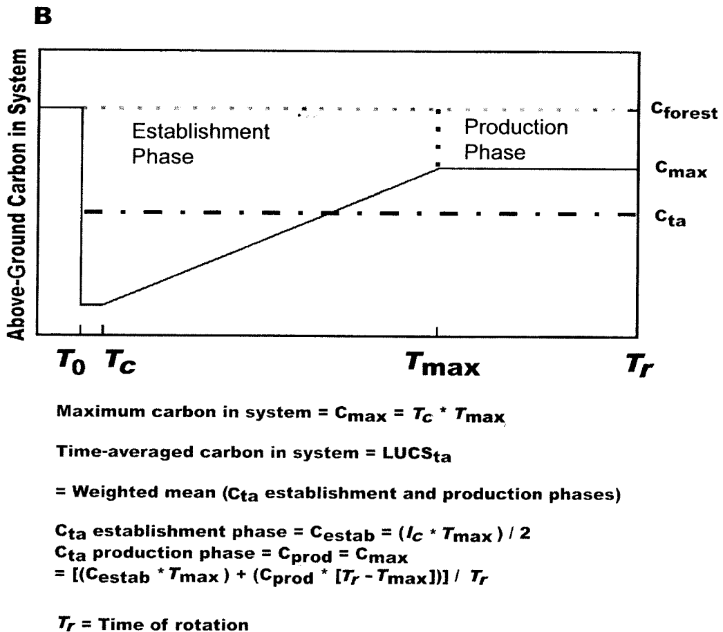
Figure 2.1 Schematic of the changes in carbon stocks and means for calculating time-averaged carbon stocks after forest clearing and establishment of (a) crop-fallow systems and (b) tree plantations.
