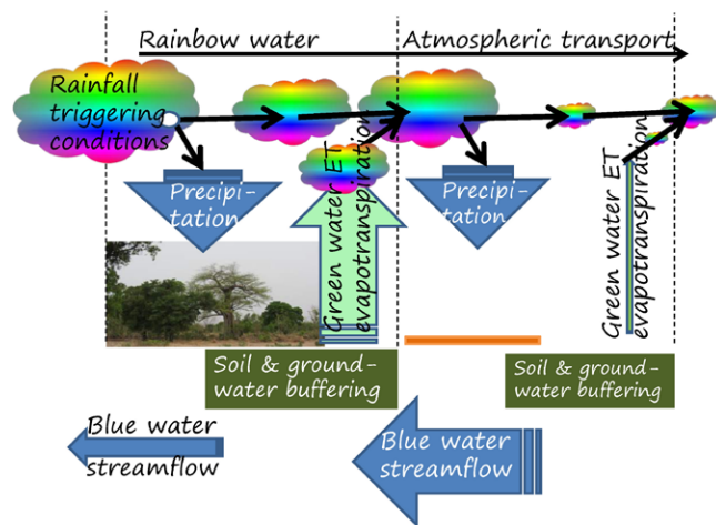
Figure 10. Interaction of small hydrological cycle, recycling 'green water', and the large ocean-land cycle with return flow through the 'blue water' of rivers 22
