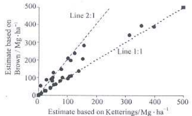
Fig. 3. Comparison of the aboveground biomass estimates based on the (generic tropical forest) 111 allometric equation and estimates based on the equation 131 that accounts for the wood density of the tree species (using the mid range estimates from a broad literature data review).
